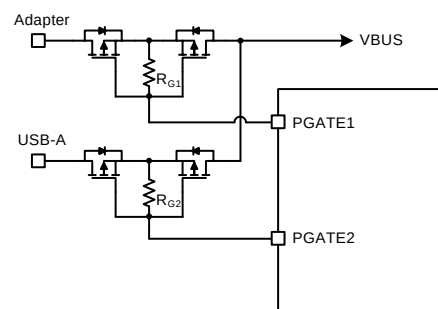
Figure 5. PGATE1/PGATE2 connection
