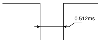
Figure 12. Interrupt pulse at /INT pin
